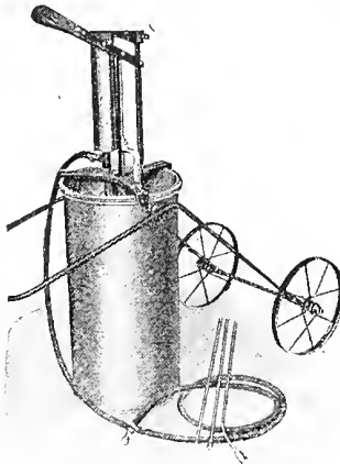
No. 3 Paragon Sprayer
